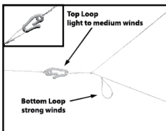
Attach the QuikClip® to the Bridle Loop. Top Loop for light to medium winds, Bottom Loop for strong winds.
